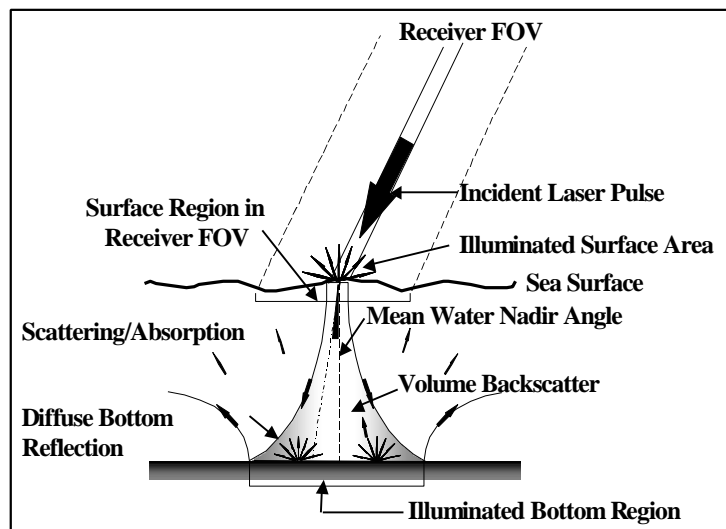
Figure 4. Water column and interface effects on system performance (FOV is field of view).
