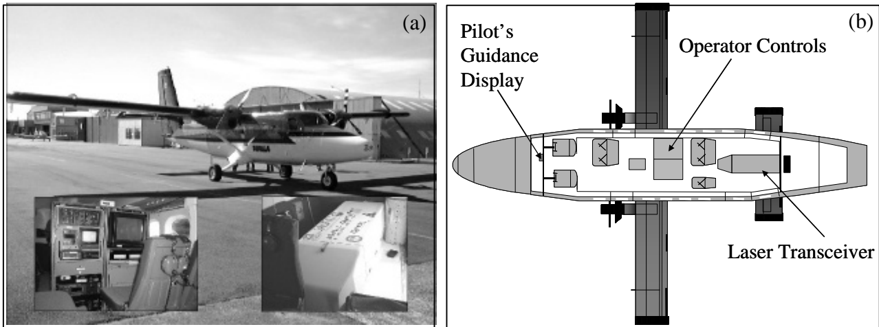
Figure 5. (a) SHOALS system mounted on a Twin Otter and (b) layout of SHOALS system inside.
