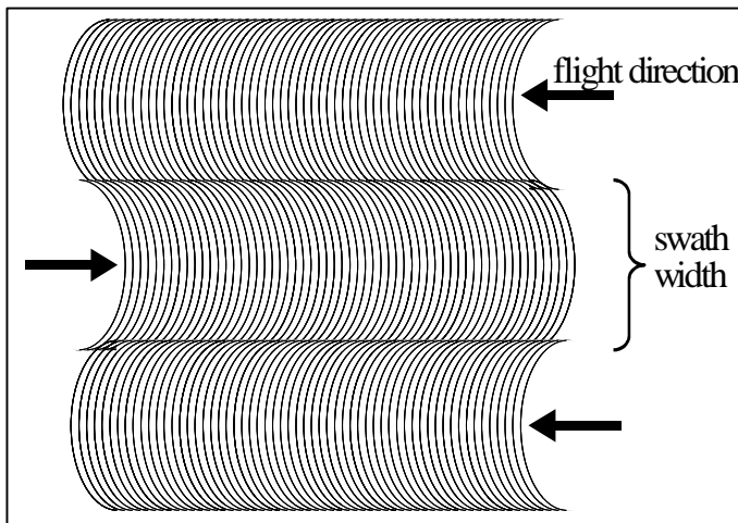
Figure 6. SHOALS scan and flight patterns.
