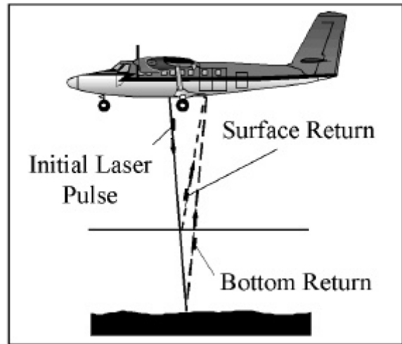
Figure 3. ALB operating principle.
